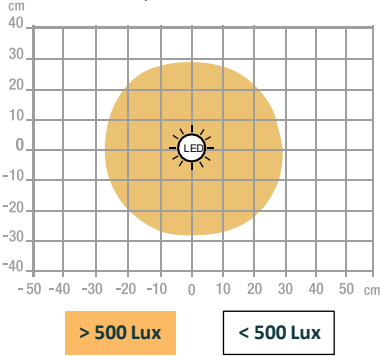
Lux measurement on the work surface in top view at 35 cm:
